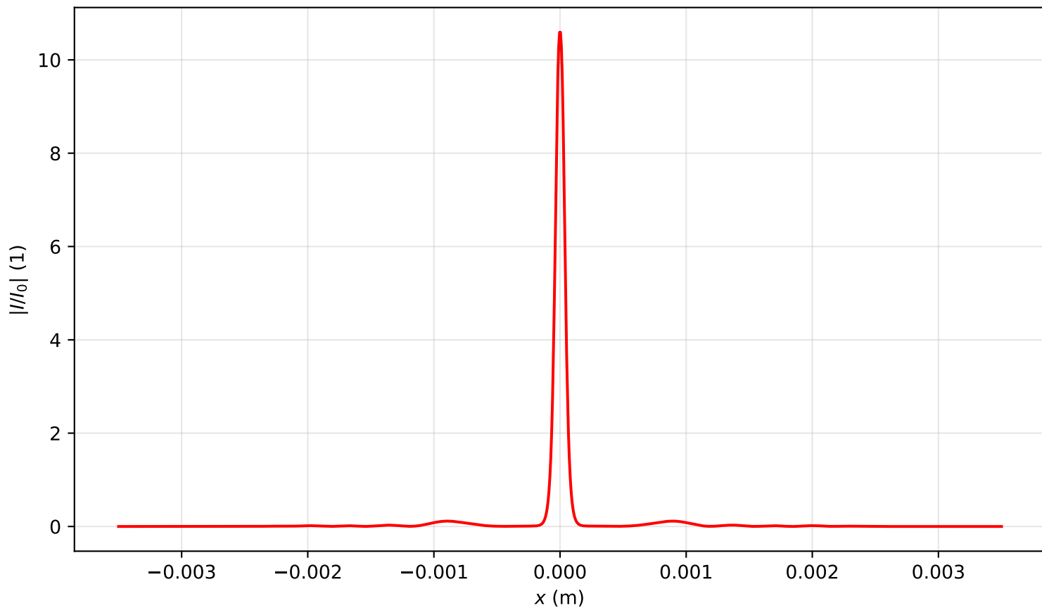
Intensity profile I(x, y = 0, z = 0.637)/I_0 , P_{in}=6.0P_{cr} , artificial time
